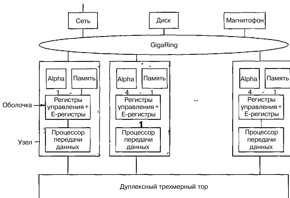
Рис. 8.29. Cray Research T3E
